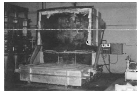
Clamshell Furnace
